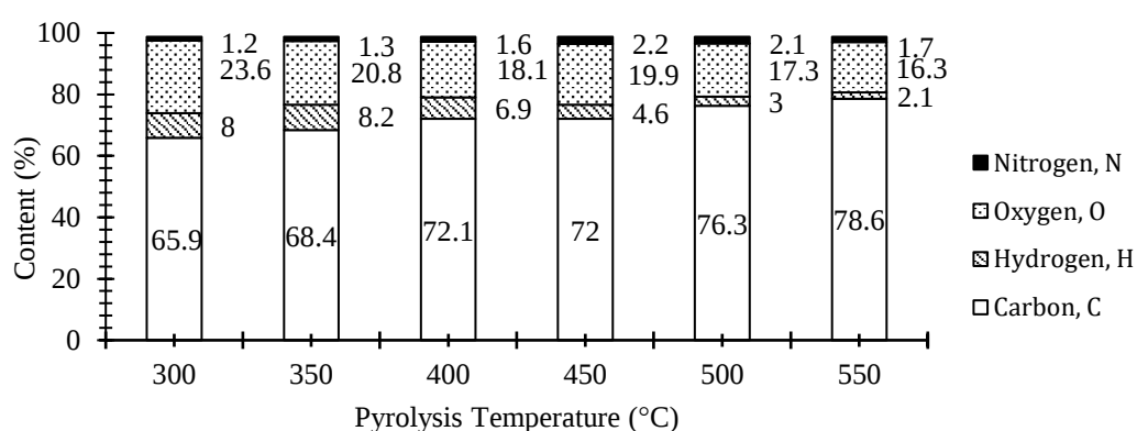
Figure 2 Carbon, Hydrogen, Oxygen and Nitrogen Content (%) against Pyrolysis Temperature (°C)
