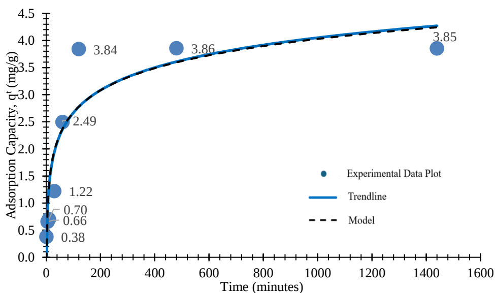
Figure 11 Adsorption Capacity, q_t (mg/g) against Contact Time (minutes) in comparison with Pseudo Second Order Model
