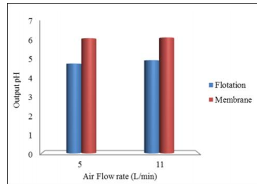
Figure 2 pH of POME after flotation without and with MBR [10]
