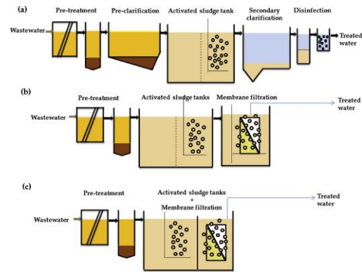
Figure 1 (a) conventional wastewater treatment process, (b) Side stream MBR (c) submerged MBR [3]
