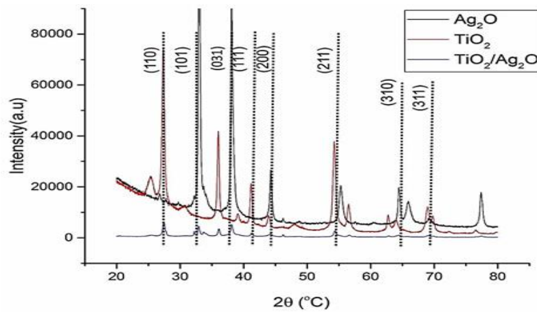
Figure 3 XRD patterns for \text{TiO}_2 , \text{Ag}_2\text{O} and \text{TiO}_2/\text{Ag}_2\text{O}
