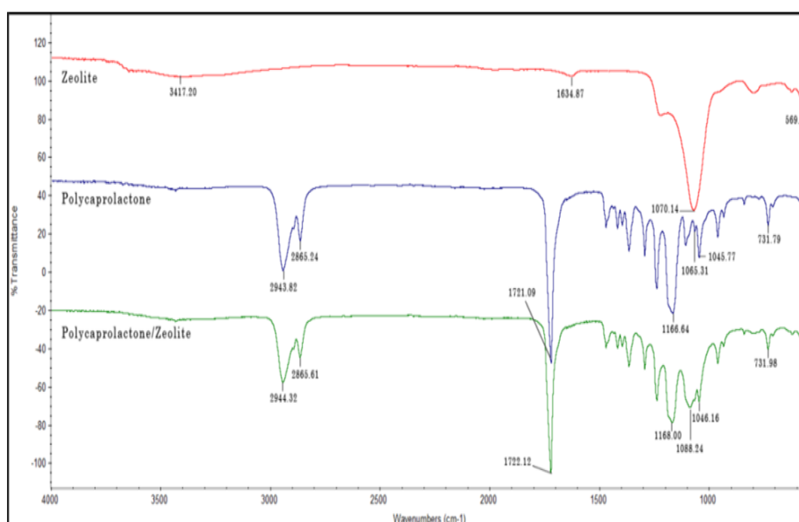
Figure 2 ATR-FTIR Spectrums for zeolite powder, PCL membrane and PCL/Zeolite membrane
